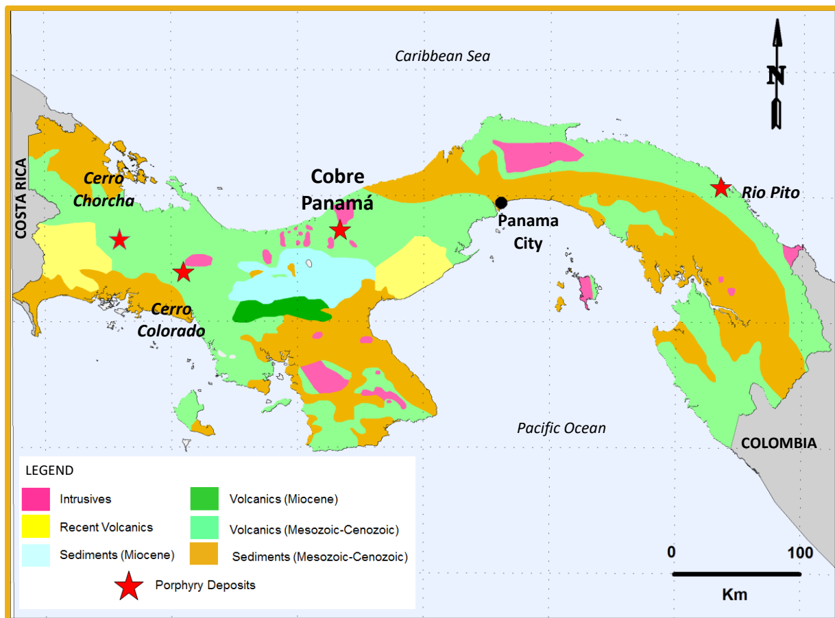
Figure 7-2 Regional geology of Panamá (source: MPSA, 2014)
