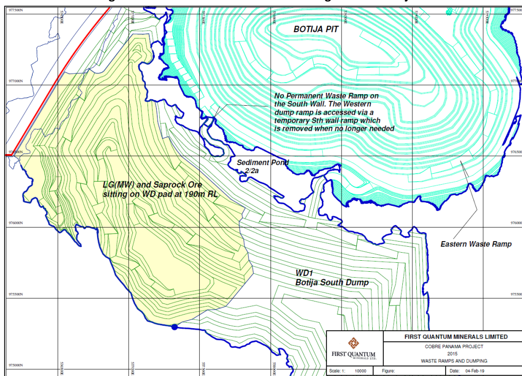
Figure 16-7 Current south wall design for the Botija Pit
