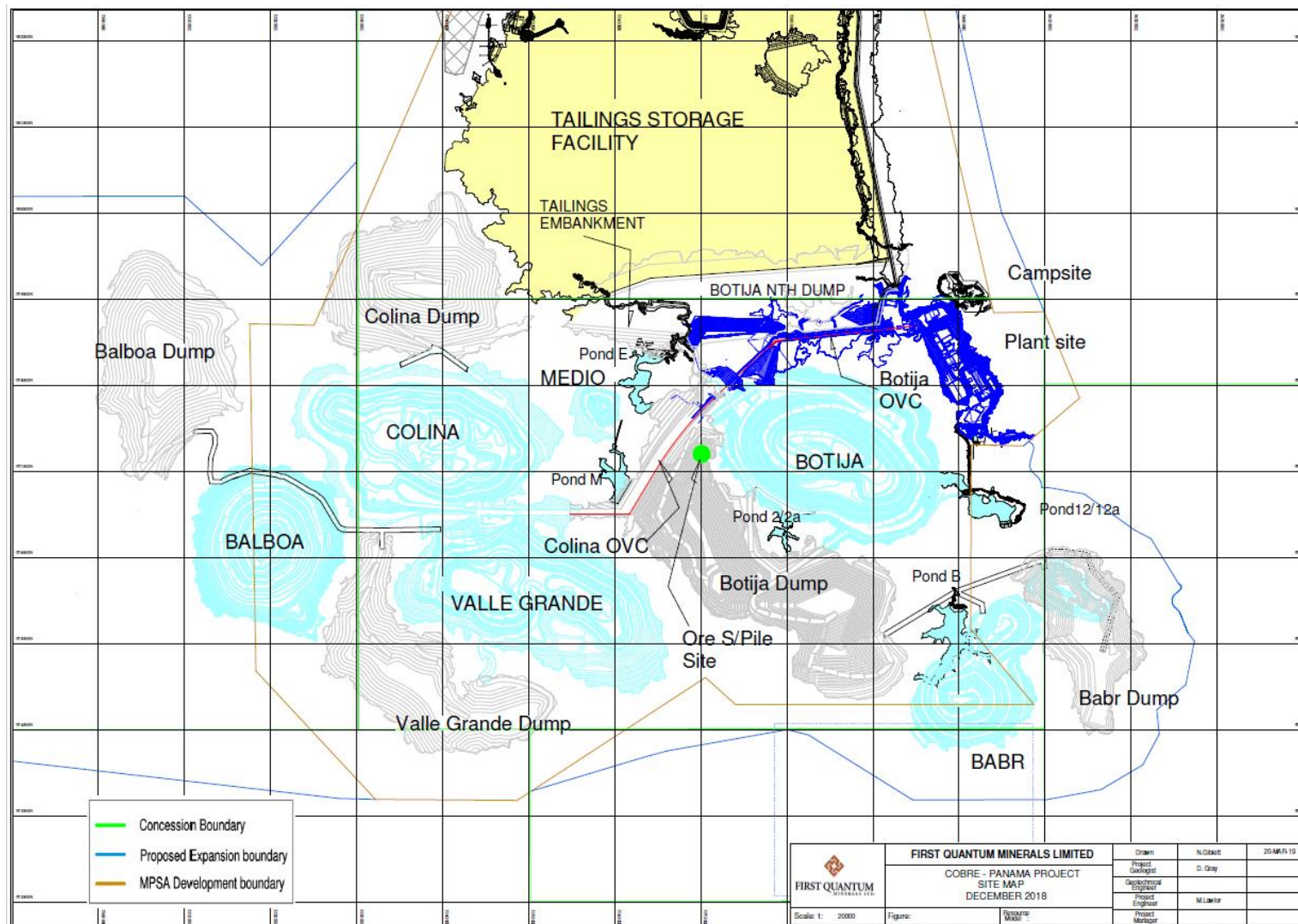
Figure 18-6 Mining facilities
