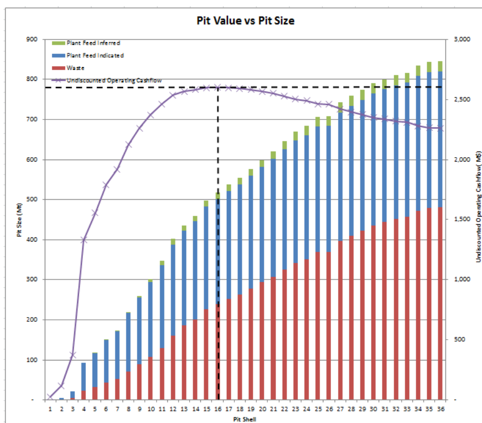
Figure 15-6 Botija Abajo, Brazo (BABR) Pit optimisation results
