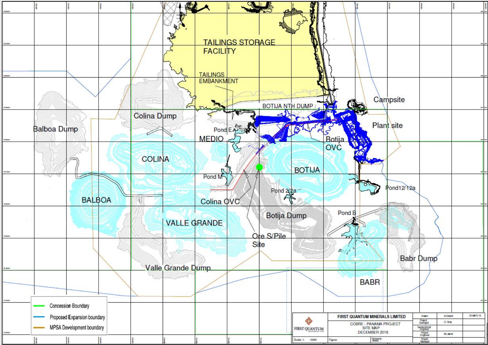
Figure 5-2 Cobre Panamá site map
