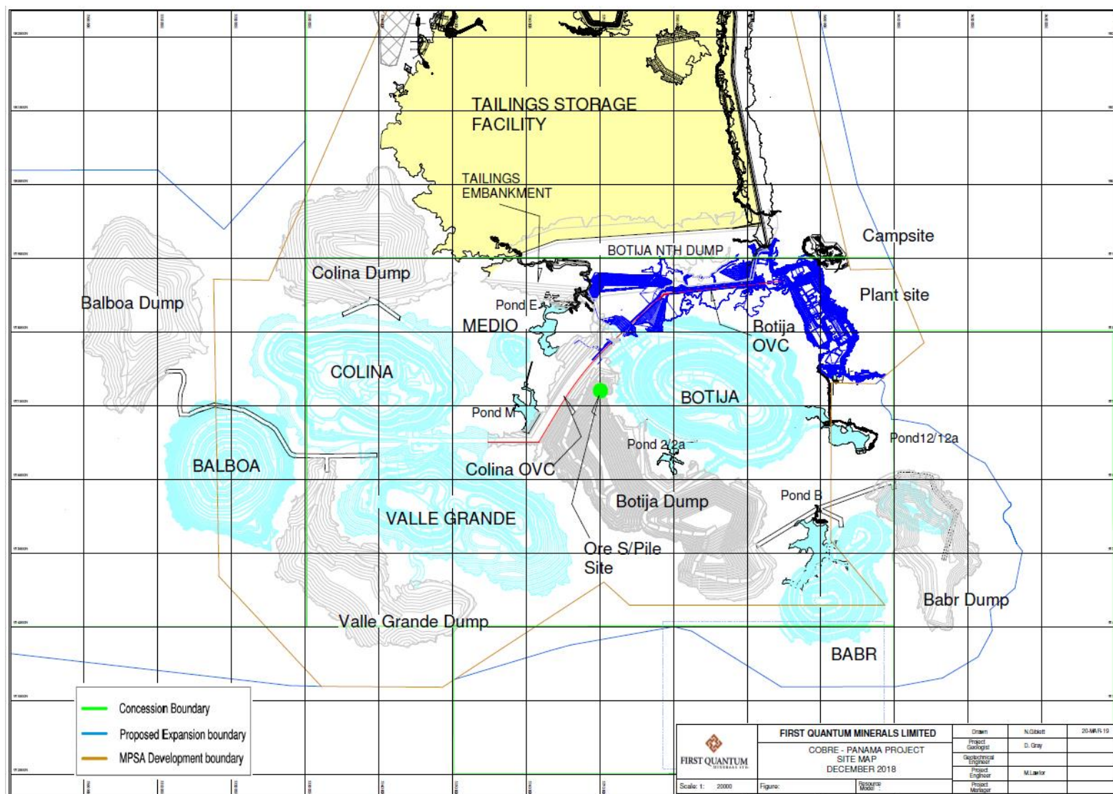
Figure 15-12 Ultimate pit designs and waste dumps
