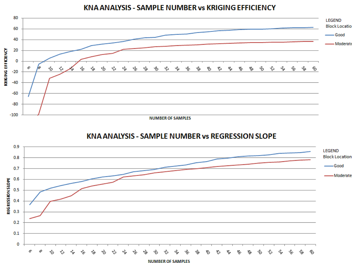
Figure 14-16 Kriging Neighbourhood Analysis to optimise sample numbers
