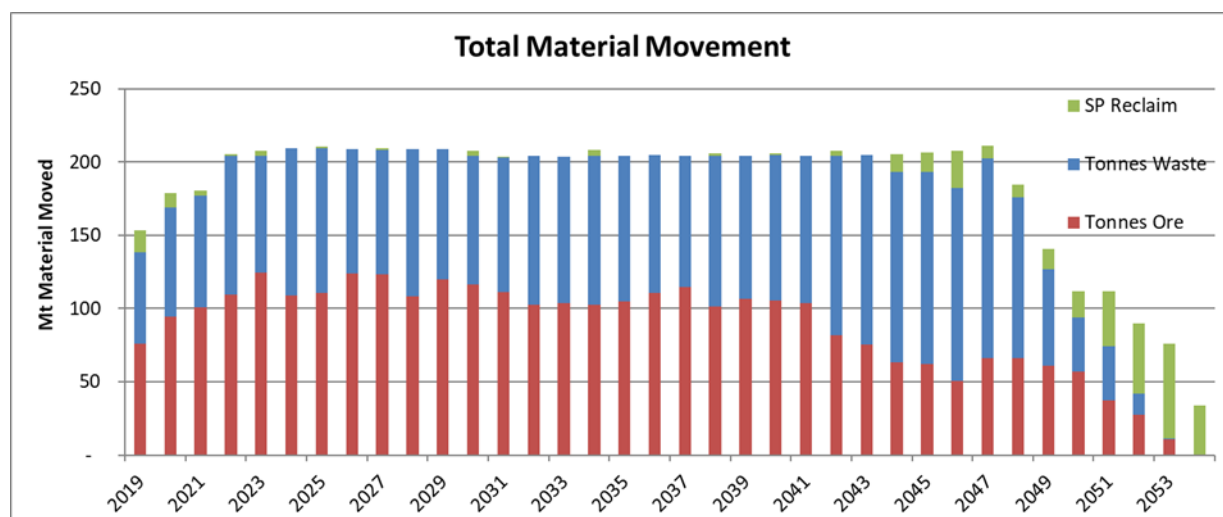
Figure 16-19 LOM scheduling – annual material movement tonnes
