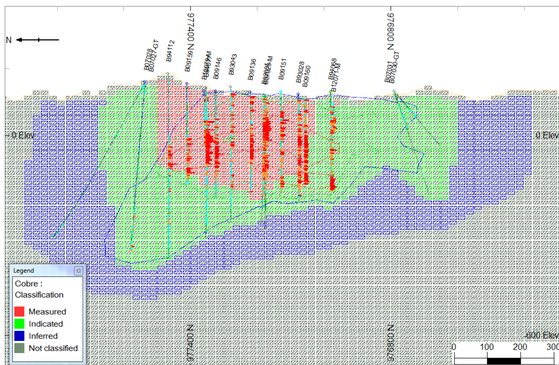
Figure 14-22 Mineral Resource classification at Botija, highlighting measured resources within closely drilled areas
