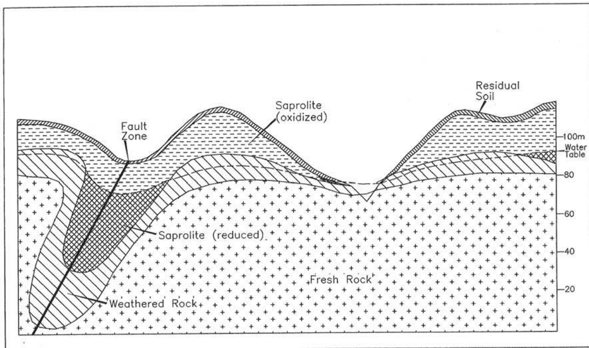
Figure 7-5 Idealised cross-section of surfaced weathering zone. Vertical scale is approximate and slightly exaggerated (from AMEC, 2007)
