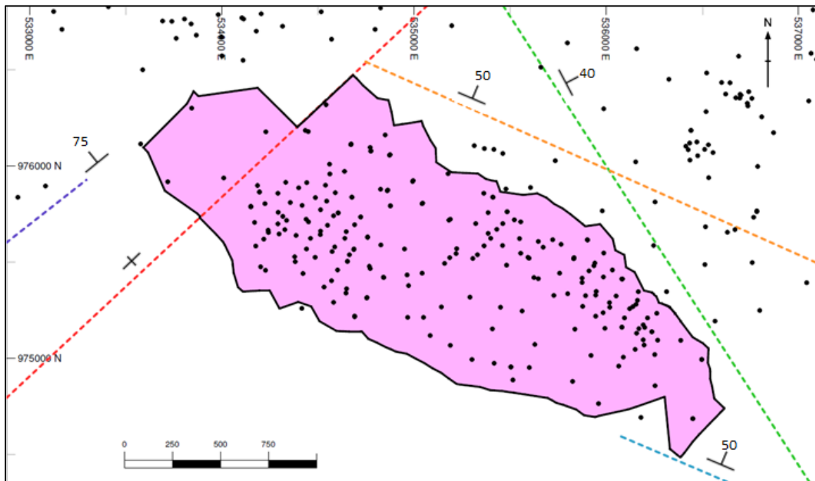
Figure 7-12 Faults identified at Valle Grande
