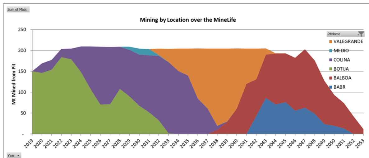
Figure 16-24 Graph showing mining sequence
